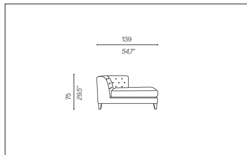
Dormeuse destra/ Right daybed Codice/Code: D80053M
